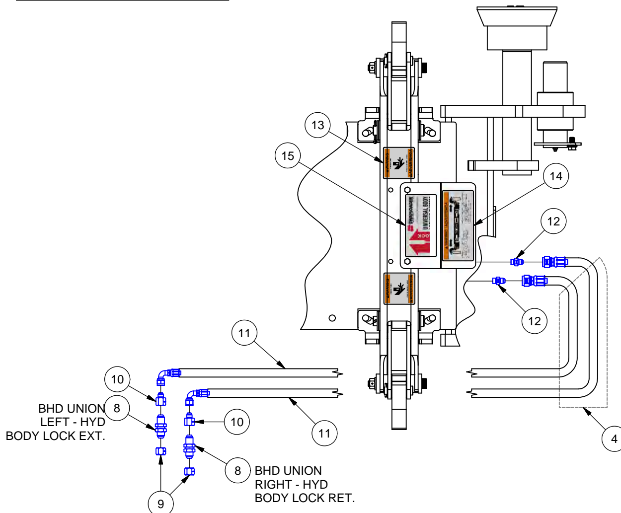
HYD BODY LOCK MOUNTING DETAIL
