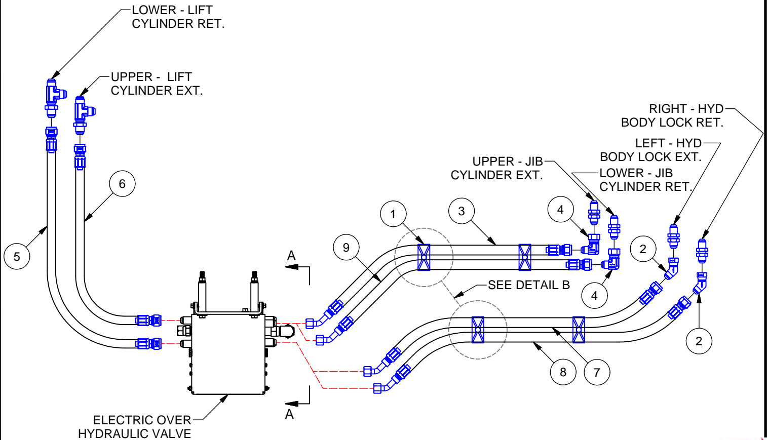
HOSE CIRCUIT, EHV 3-SECT 200S
