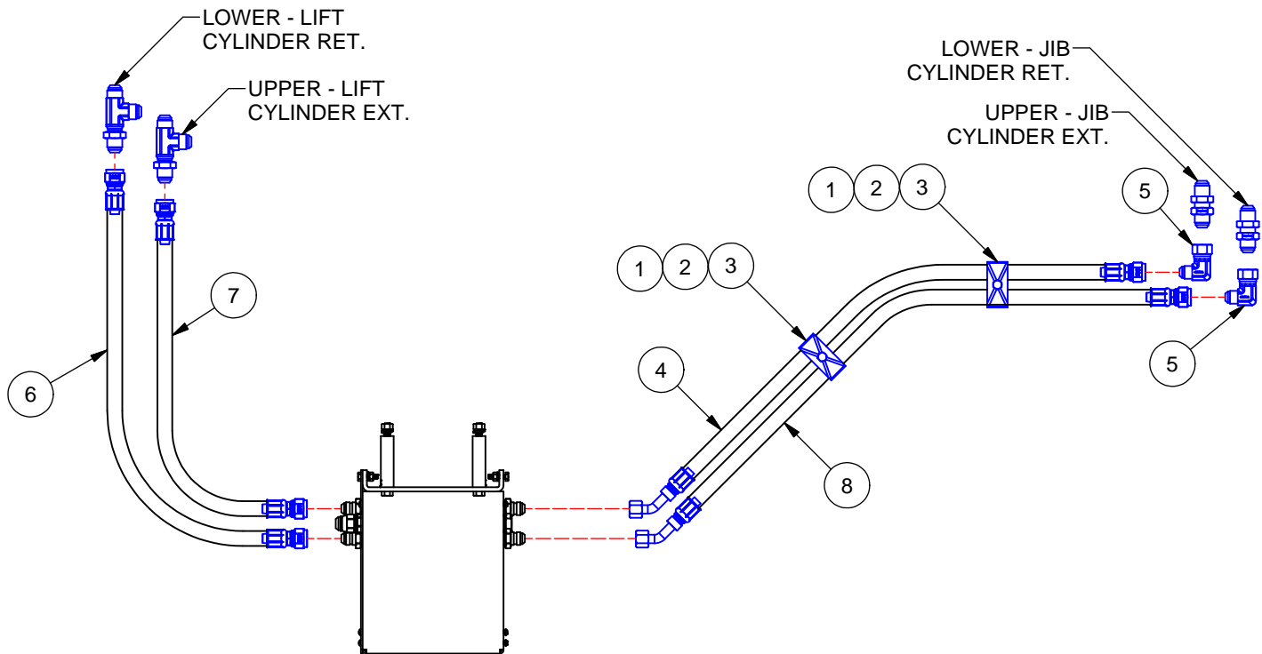
HOSE CIRCUIT, EHV 2-SECT 200S
