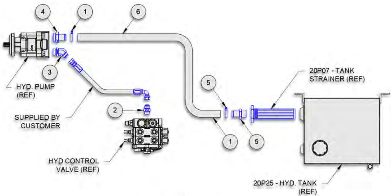
PUMP CIRCUIT
