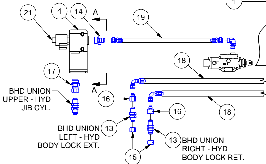
CYLINDER CIRCUIT, BL 200S STD
