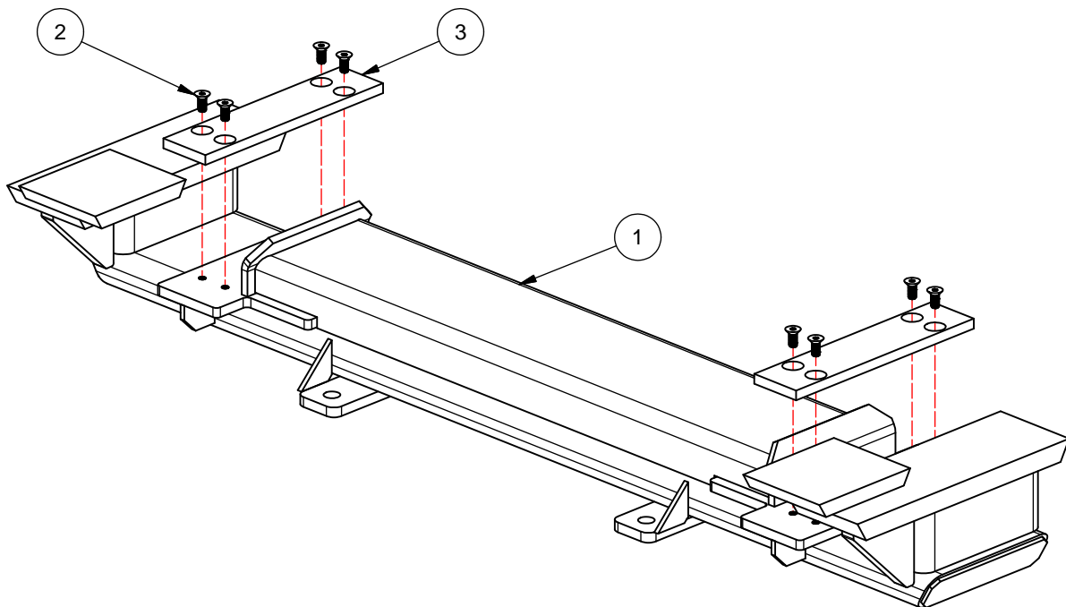
BODY LOCK W/SHELF, X-HD
