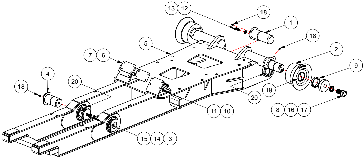
PIVOT JOINT SUB-ASSY, 518X
