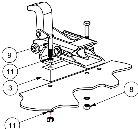
HYD BODY LOCK MOUNTING DETAIL
