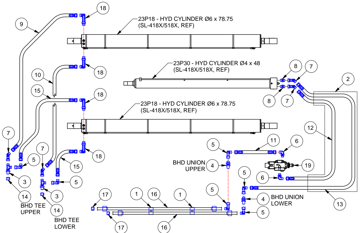
BASE CYLINDER CIRCUIT, 418X/528X
