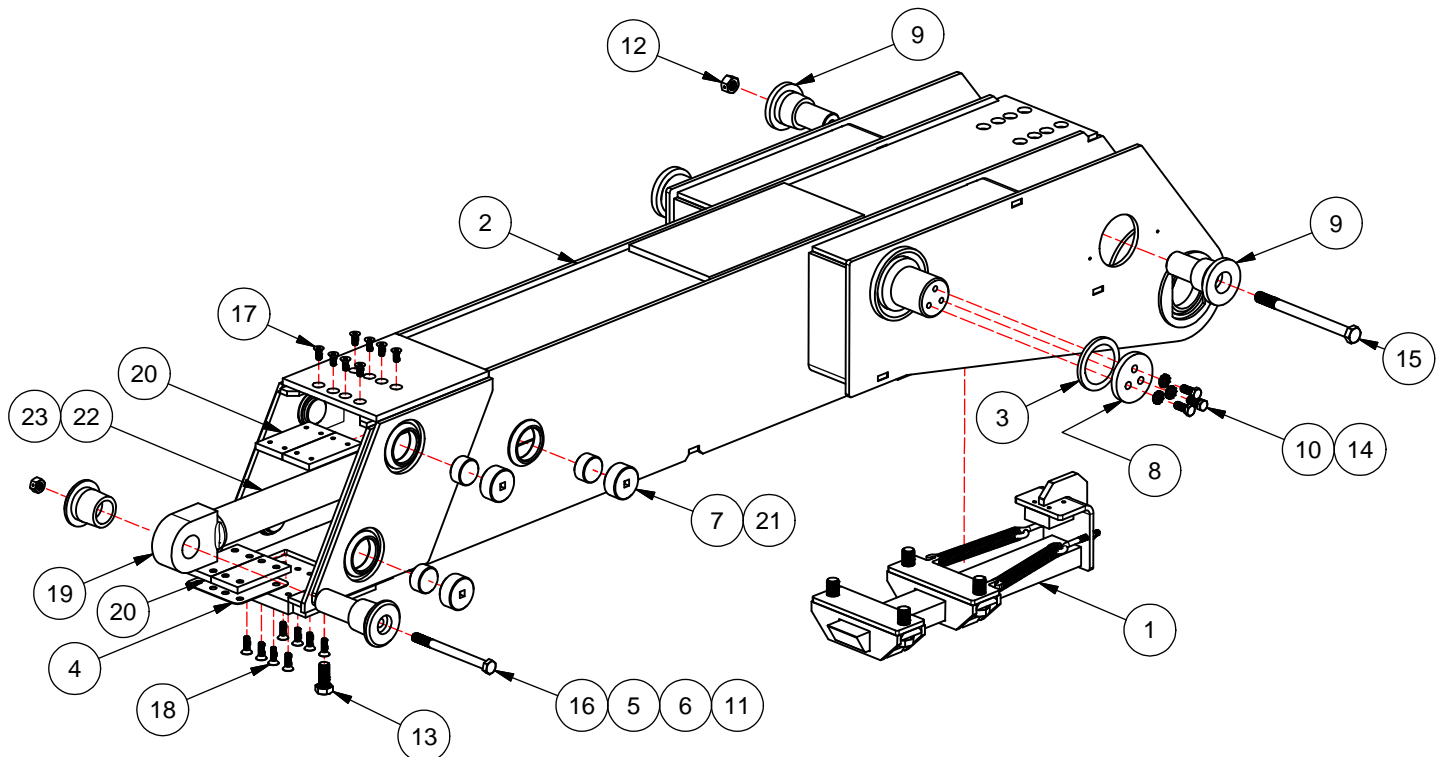
OUTER TUBE SUB-ASSY, SL-518X
