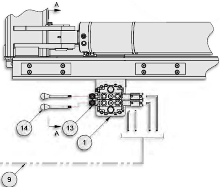
AIR CONTROLS, 2-SECTION
