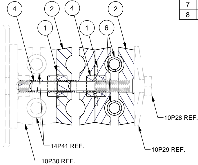
FRONT CLAMP DETAIL
