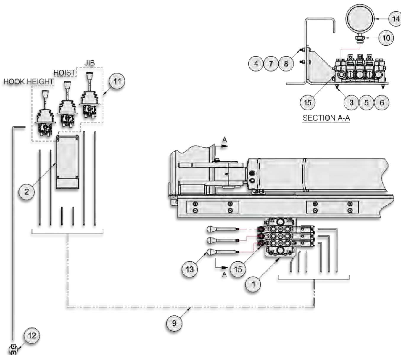
AIR CONTROLS, 3-SECTION HYD JIB
