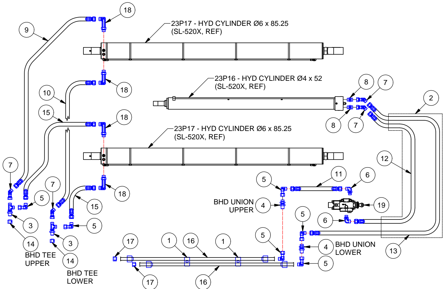
BASE CYLINDER CIRCUIT, 520X
