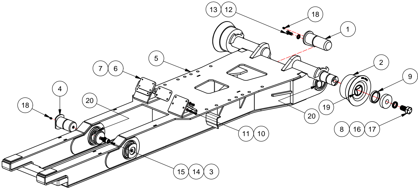
PIVOT JOINT SUB-ASSY, 520X
