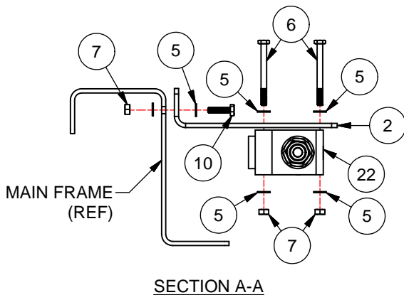
HYD BODY LOCK MOUNTING DETAIL
