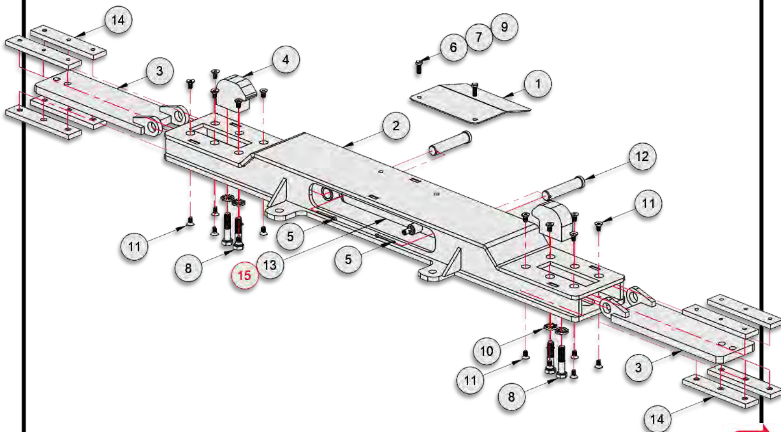
O-LOCK ASSEMBLY
