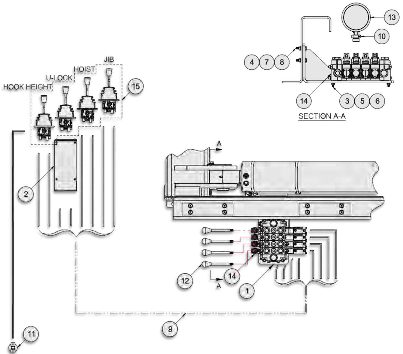
AIR CONTROLS, 4-SECTION HYD JIB
