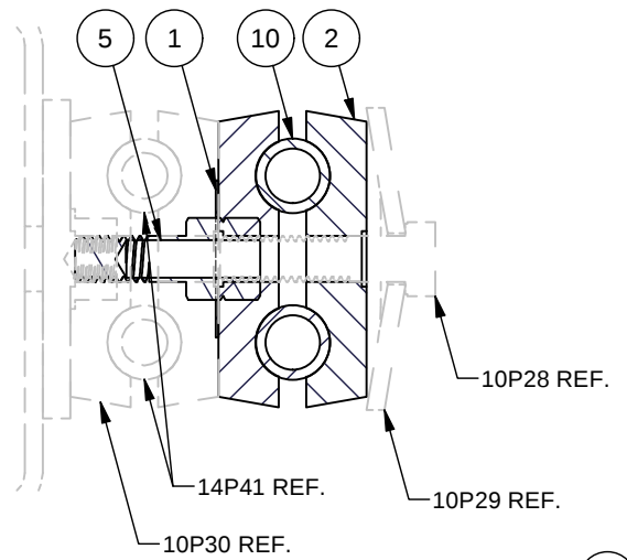
REAR CLAMP DETAIL
