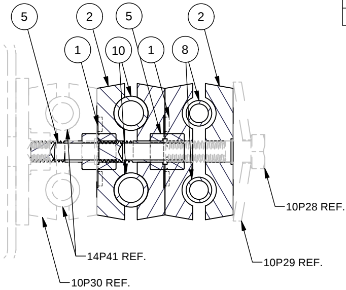
FRONT CLAMP DETAIL
