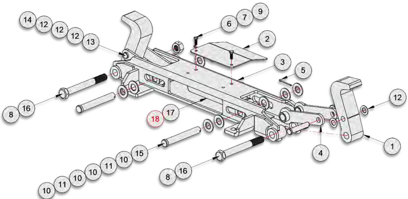
U-LOCK ASSEMBLY
