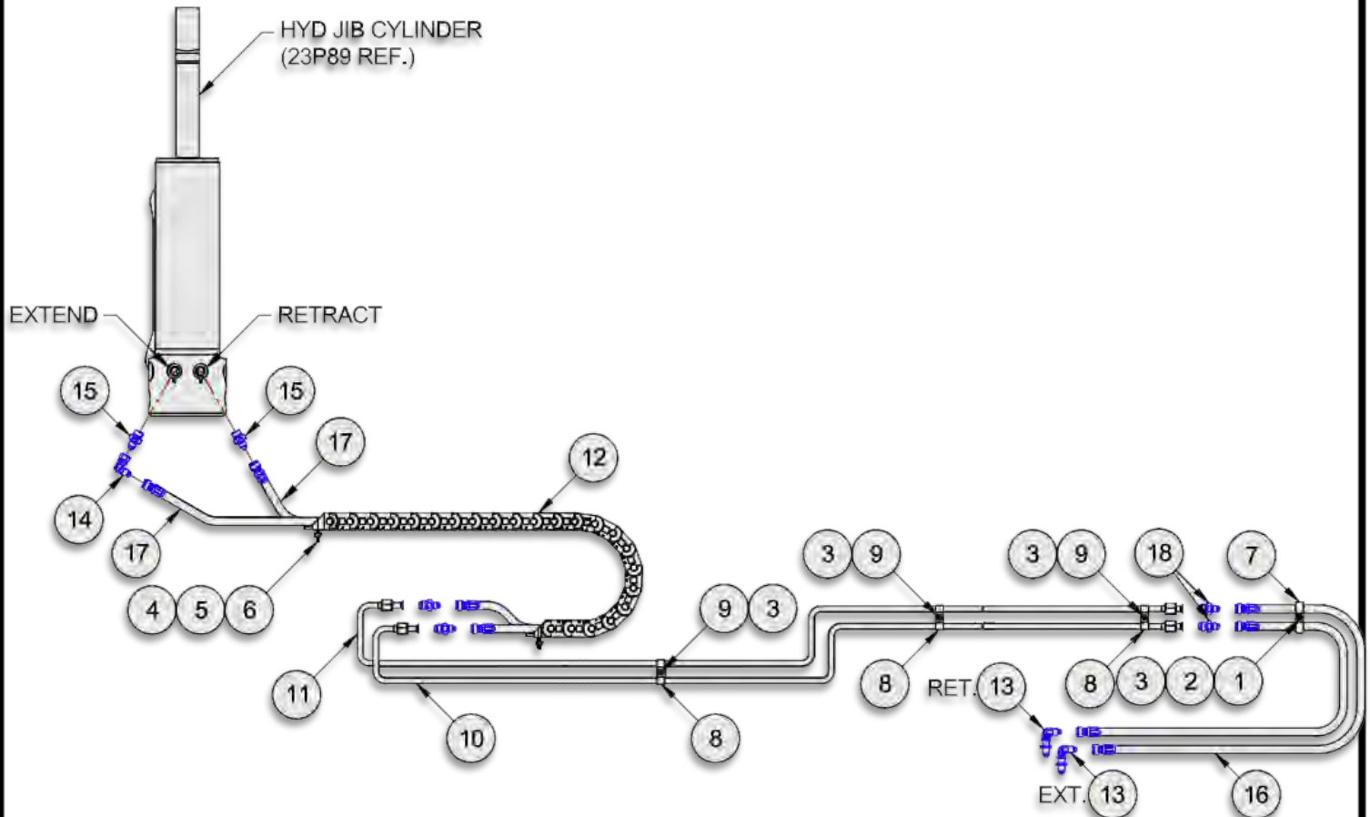
CYL CIRCUIT, HYD JIB
