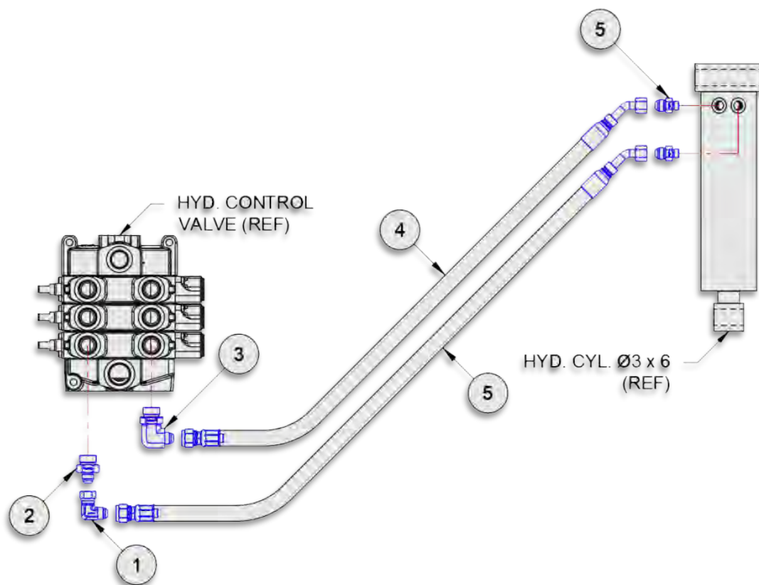
STABILIZER CIRCUIT
