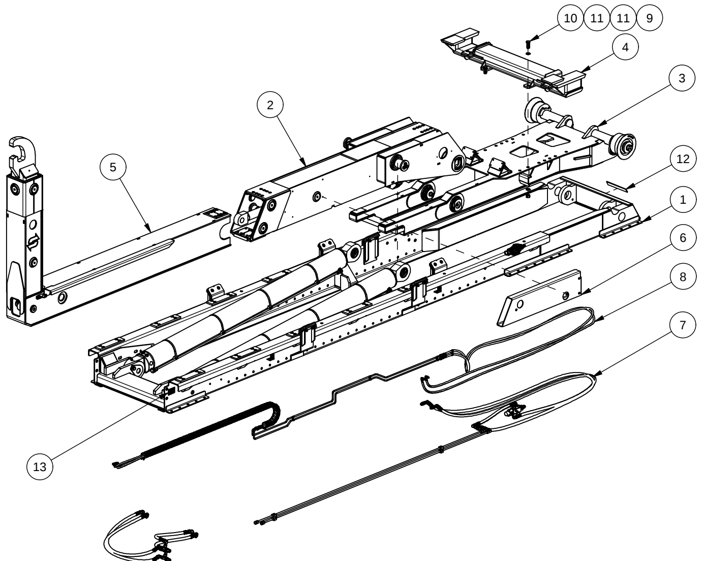
SL-520X BASE HOIST W/ HYD JIB
