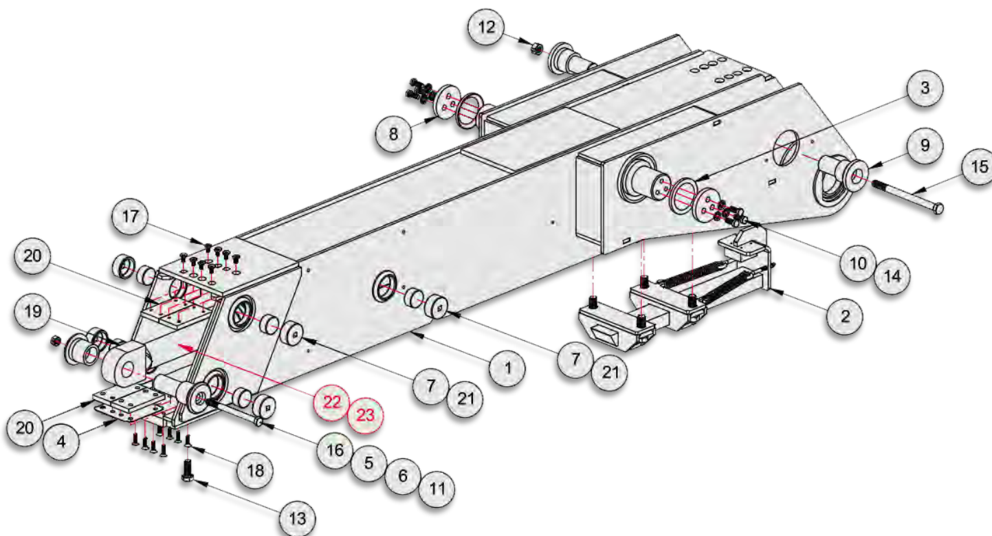
OUTER TUBE SUB-ASSEMBLY
