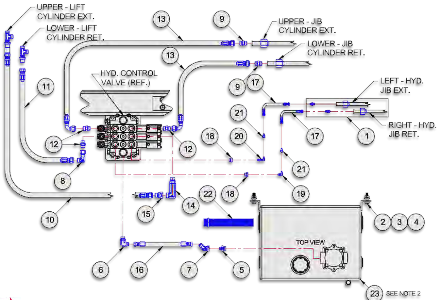
TANK CIRCUIT, 3-SECTION HJ 520X
