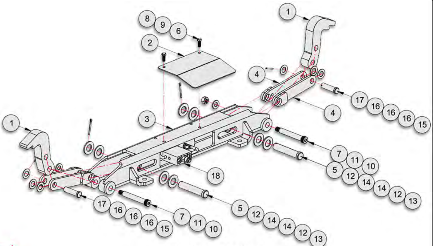
U-LOCK ASSEMBLY
