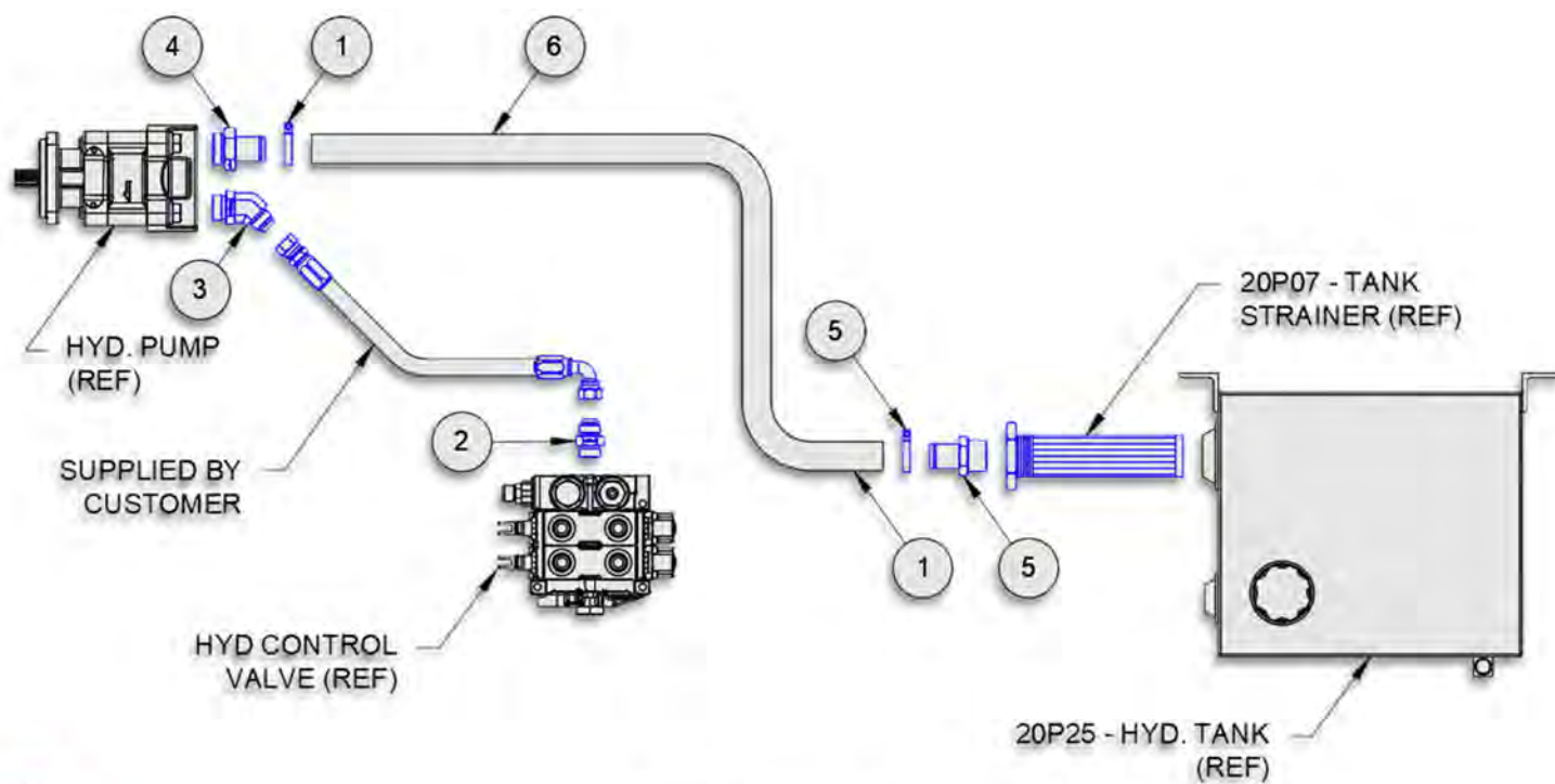
PUMP CIRCUIT
