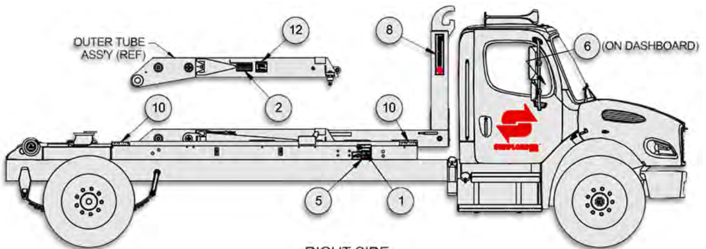
RIGHT SIDE
